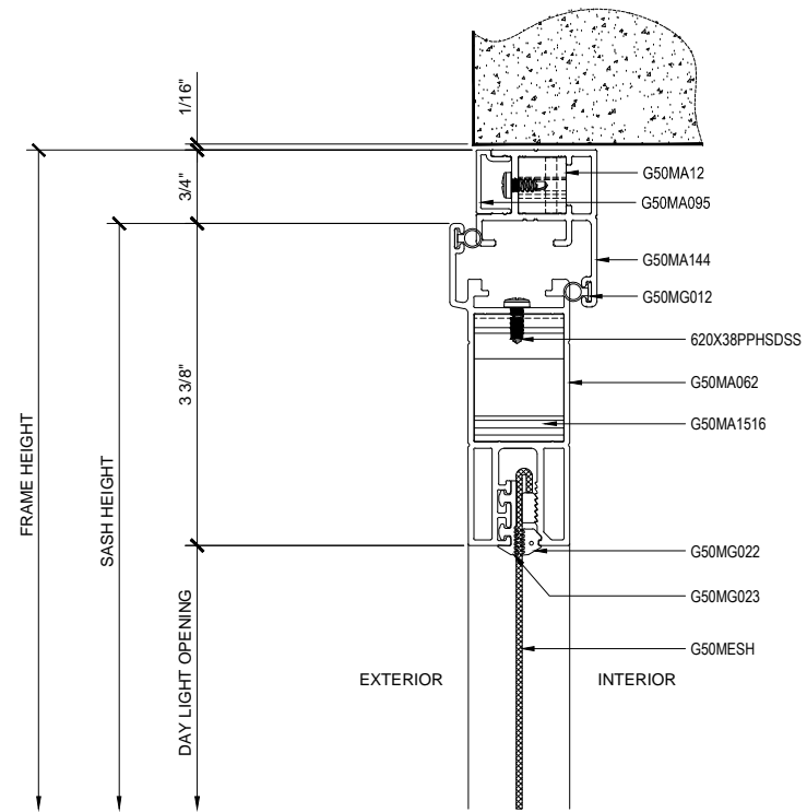
① SECTION DETAIL AT HEAD
