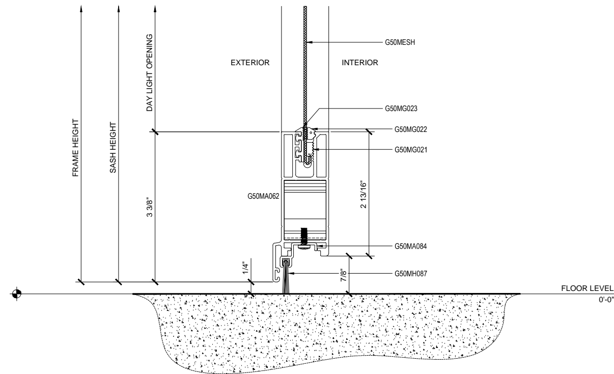
② SECTION DETAIL AT SILL
