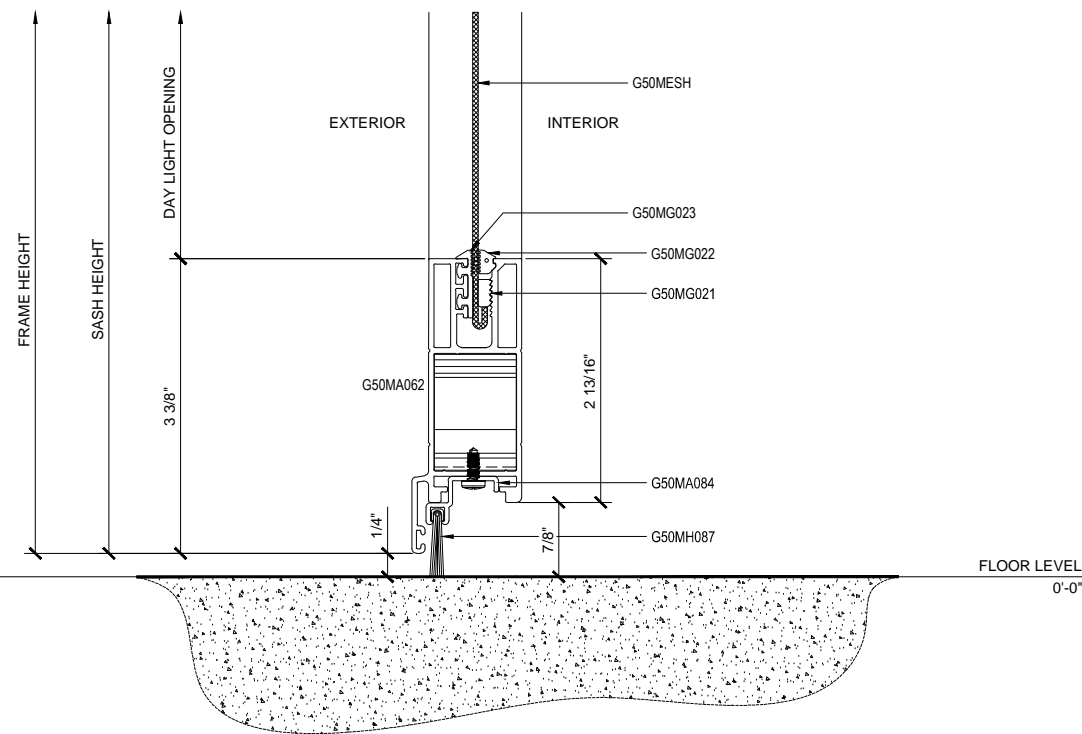
② SECTION DETAIL AT SILL
