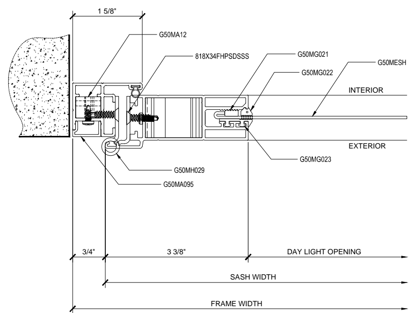
① SECTION DETAIL AT JAMB ARCH REF: N/A 1'-0"=1'-0"
