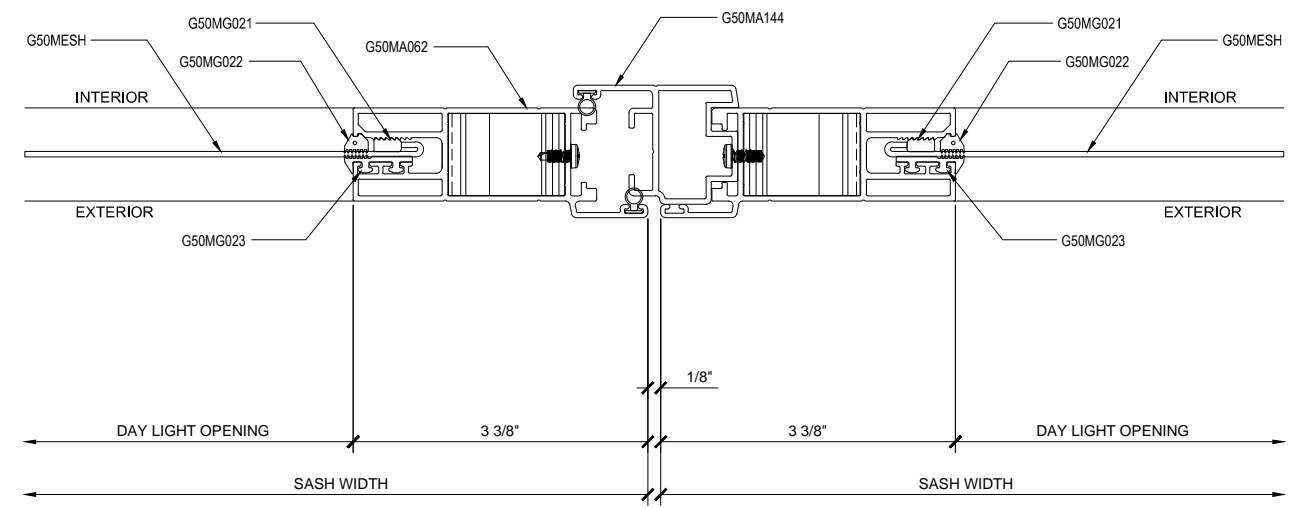
③ SECTION DETAIL AT JAMB ARCH REF: N/A 1'-0"=1'-0"
