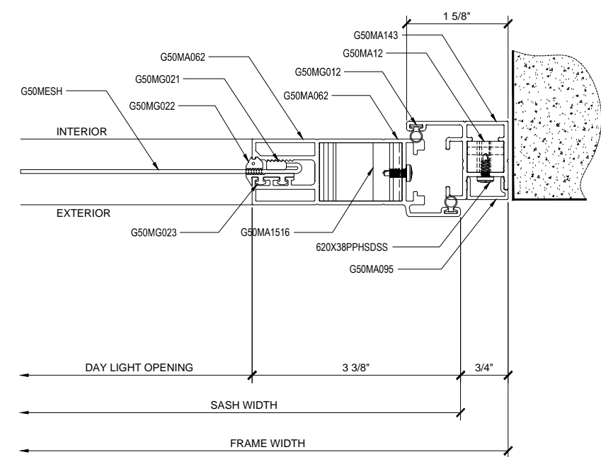
② SECTION DETAIL AT JAMB ARCH REF: N/A 1'-0"=1'-0"
