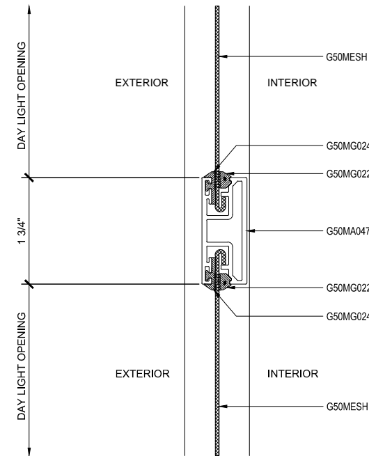
③ SECTION DETAIL AT MIDRAIL - OPTIONAL
